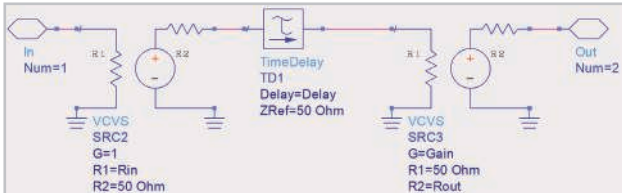
Figure 37. Time-delay subcircuit schematic.
