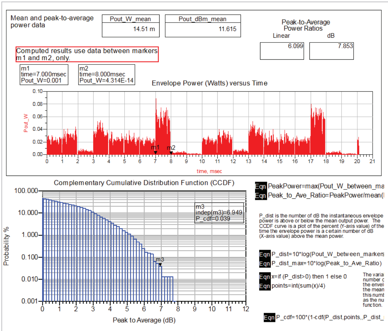
Figure 15. Setting marker locations is one way to see power data within a particular burst.
