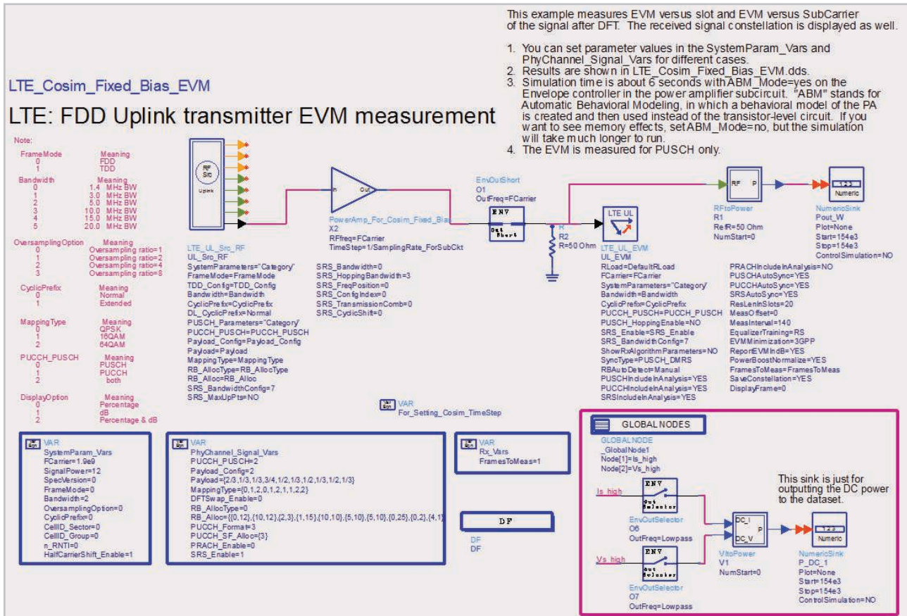
Figure 23. Ptolemy co-simulation schematic.
