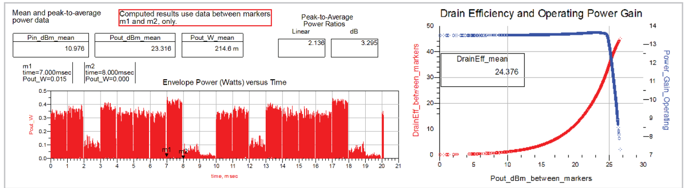
Figure 27. LTE_Cosim_Fixed_Bias_EVM_alt co-simulation data from 7 to 8 msec.
