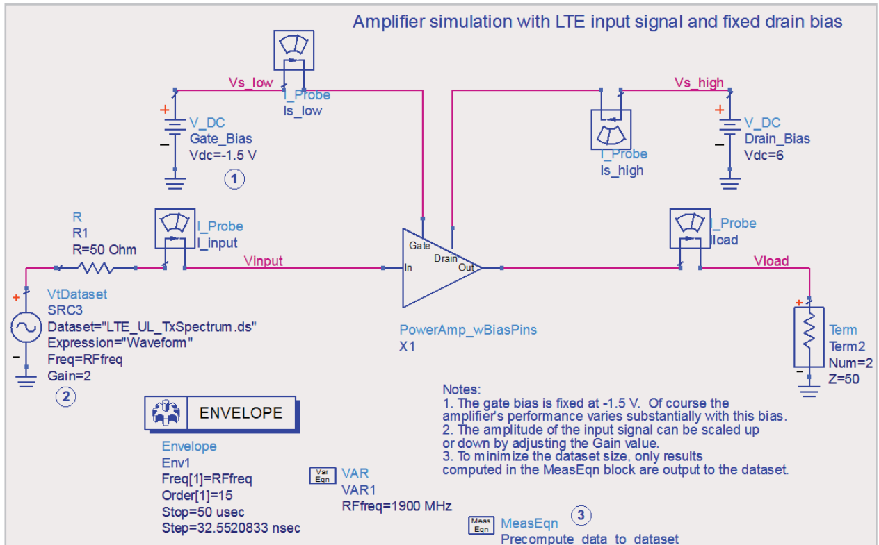
Figure 16. Simulating the power amplifier with a fixed drain bias.
