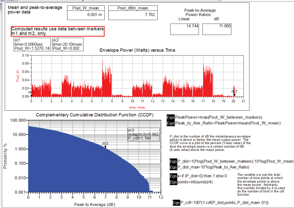
Figure 14. The LTE_Source_Test data display.
