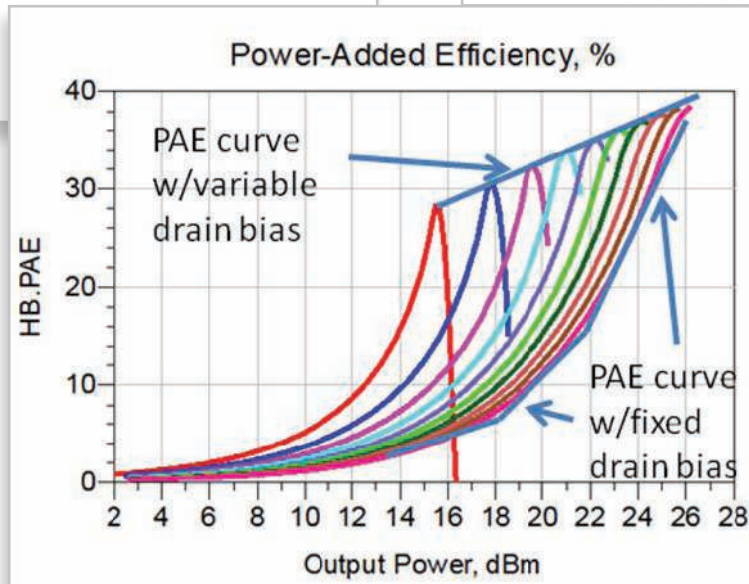
Figure 2. Higher PAE can be attained if the PA's drain bias can be adjusted dynamically along with the input signal magnitude.
