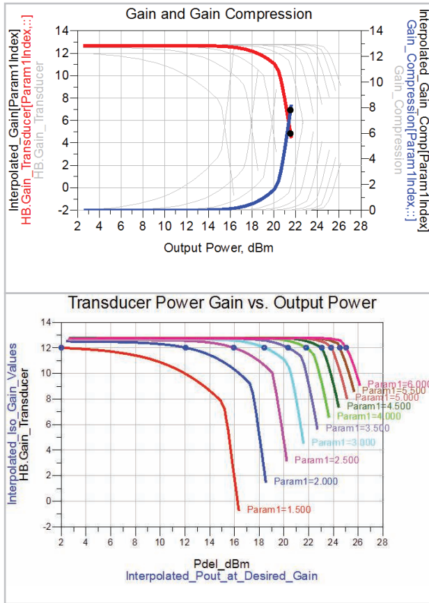
Figure 8. Plot of gain and gain compression.
