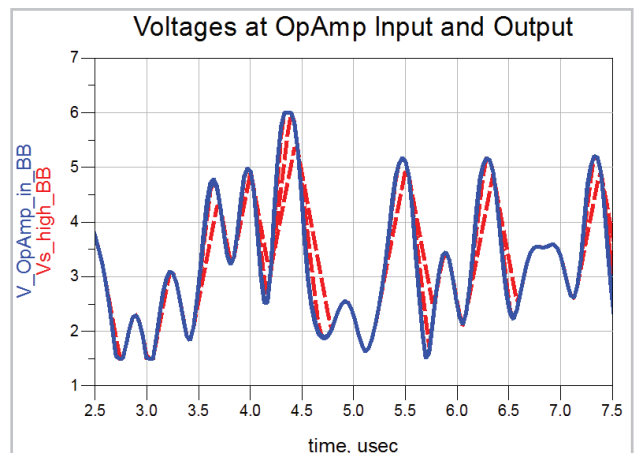
Figure 34. Plot showing slew rates of the drain bias voltage.
