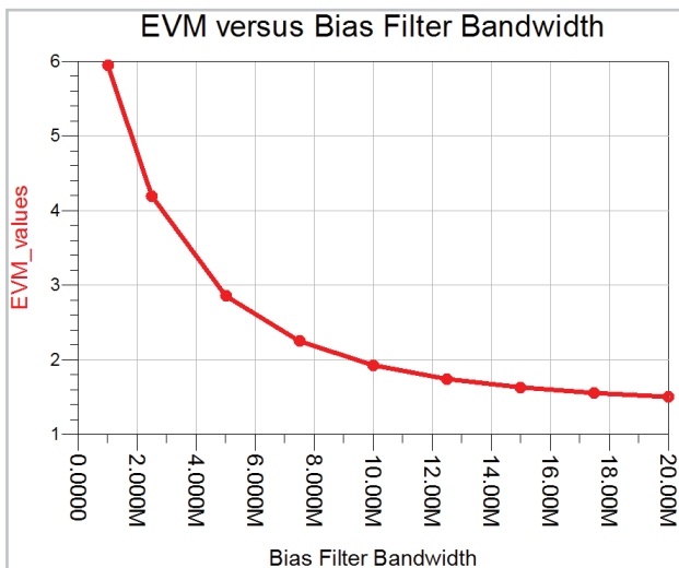
Figure 41. Plot of raw EVM data versus bias filter bandwidth.
