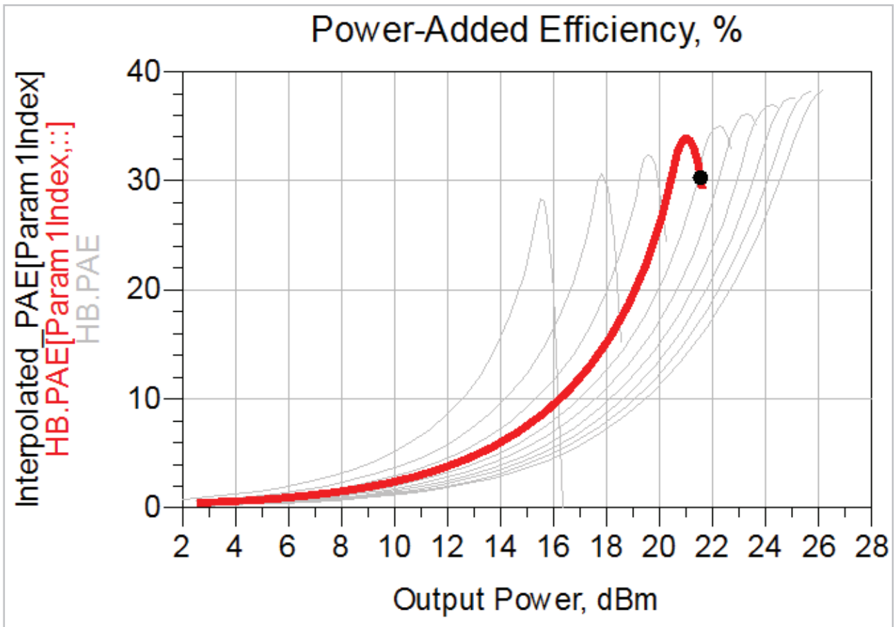
Figure 7. Plot of PAE versus output power, showing increasing drain bias from left to right.
