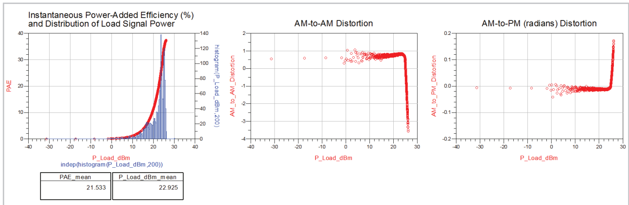
Figure 20. Fixed bias simulation with Gain=2.5 on the LTE source.
