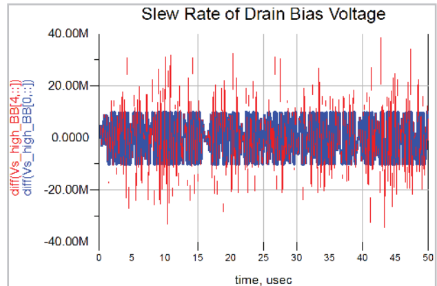
Figure 34. Plot showing slew rates of the drain bias voltage.
