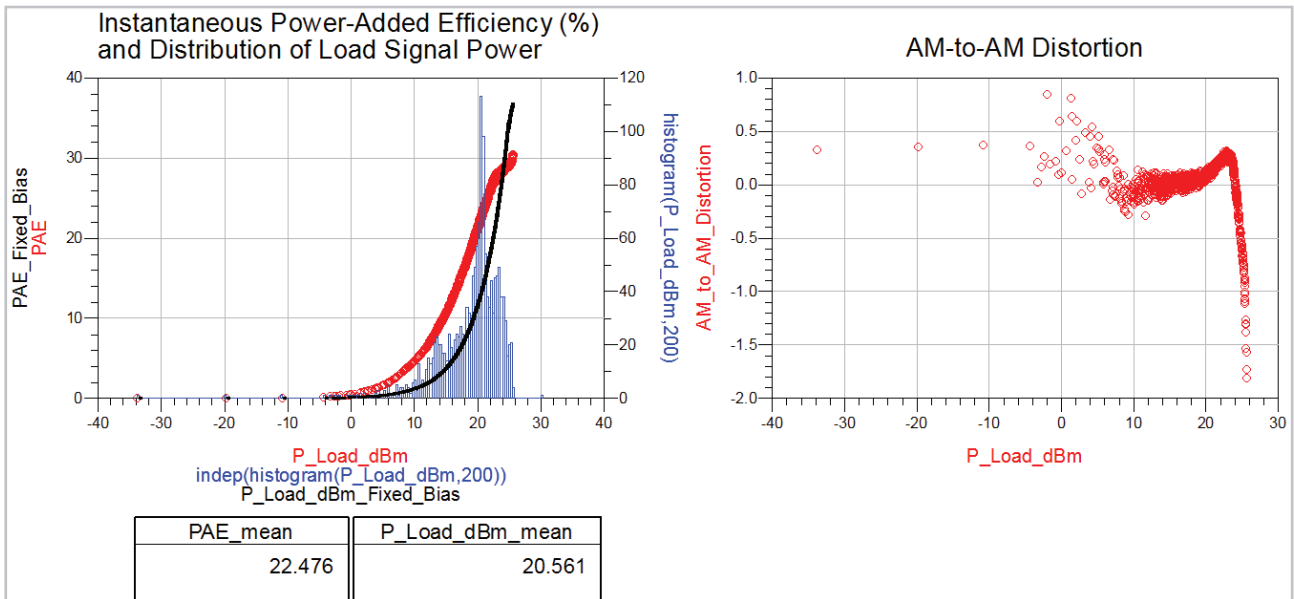
Figure 22. ET simulation using a shaping table to maintain 11 dB constant gain.
