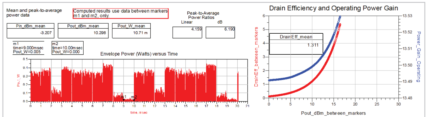
Figure 28. LTE_Cosim_Fixed_Bias_EVM_alt co-simulation data from 9 to 10 msec.
