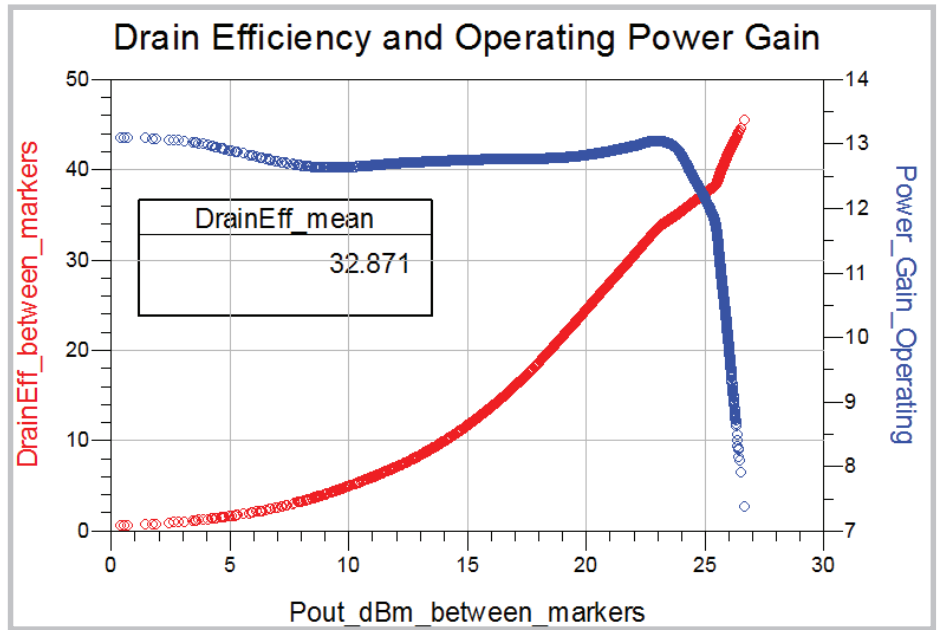
Figure 30. Drain efficiency and operating power gain during the 7 to 8 msec. burst, with ET on.
