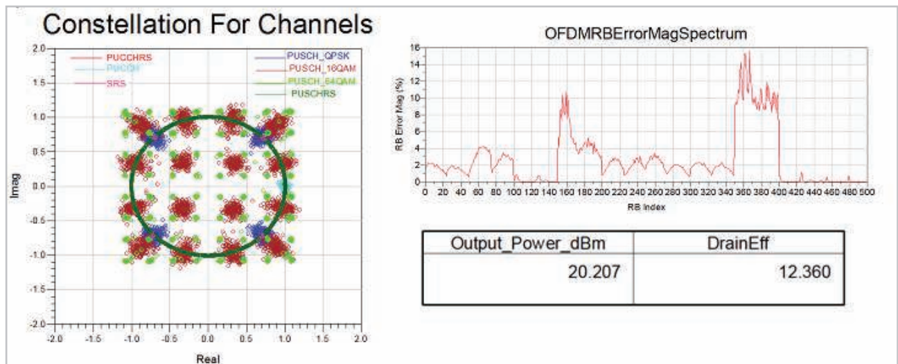
Figure 24. Ptolemy co-simulation results.
