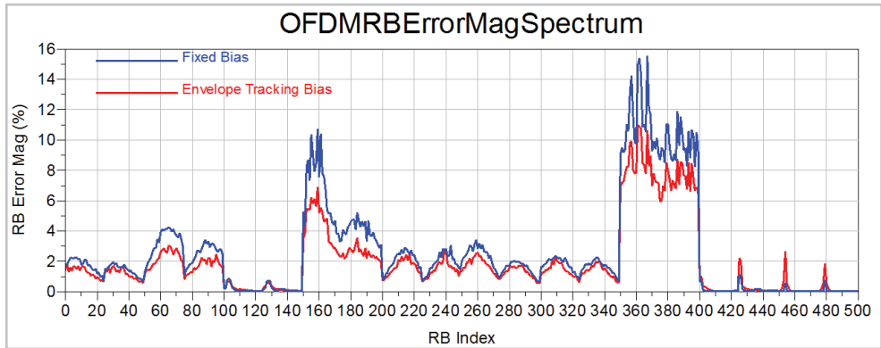
Figure 29. Ptolemy co-simulation results with ET employed.
