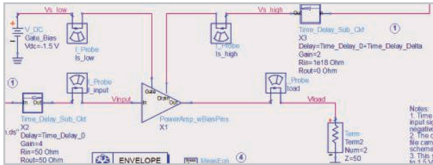
Figure 36. Schematic for modeling timing skew effects
