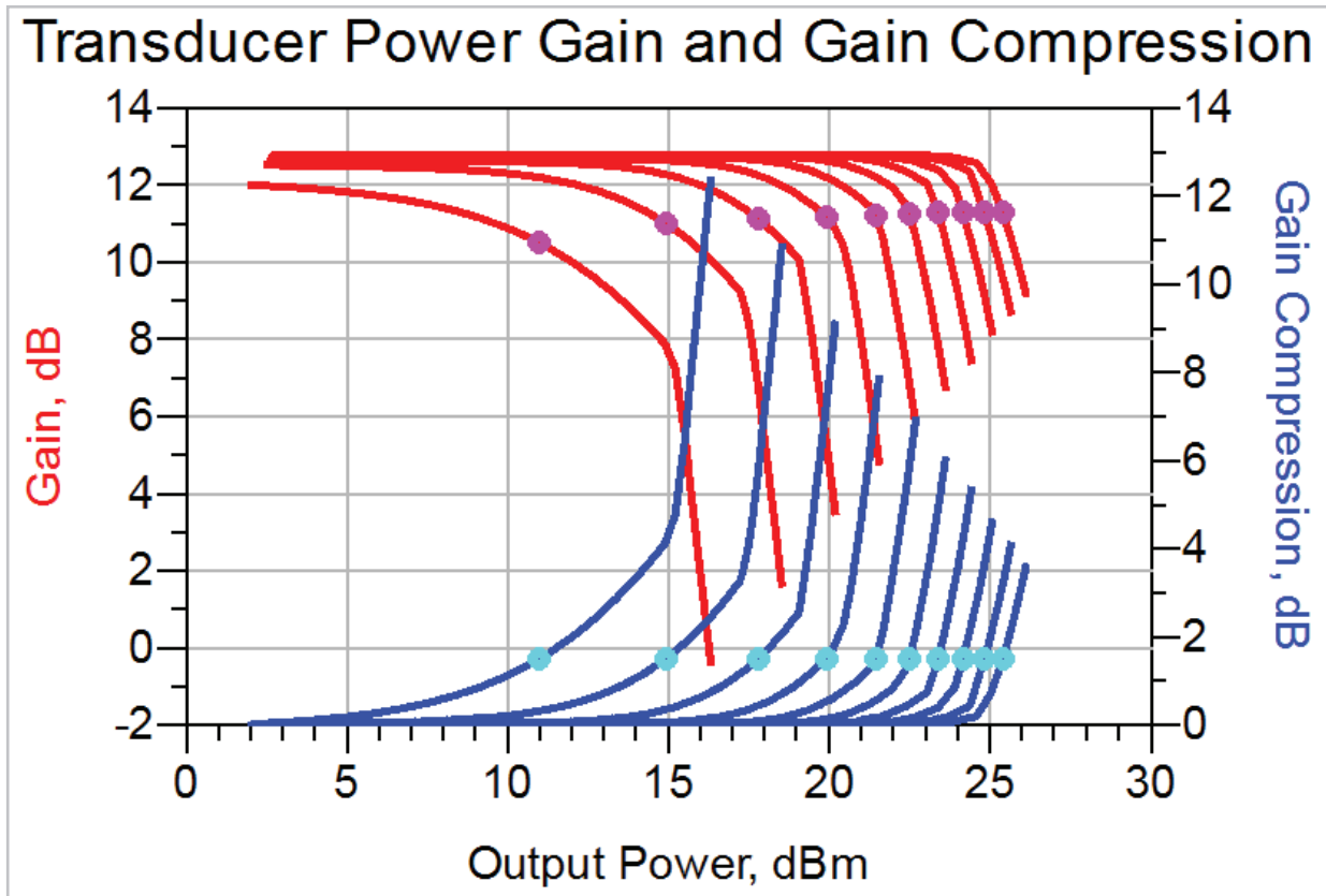
Figure 11: Interpolated values at 1.5 dB of gain compression.
