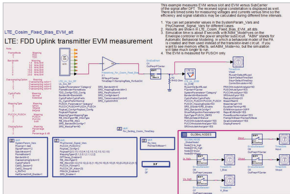
Figure 25. LTE_Cosim_Fixed_Bias_EVM_alt co-simulation schematic.
