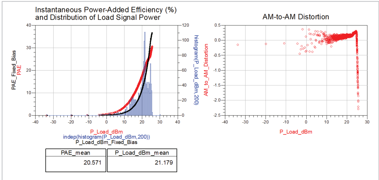
Figure 19. Simulation results after applying ET.
