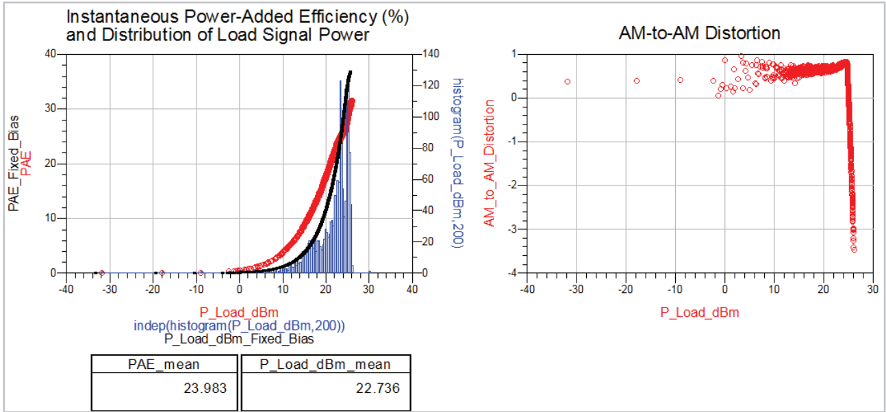
Figure 21. ET simulation with Gain=2.5 on the LTE source.
