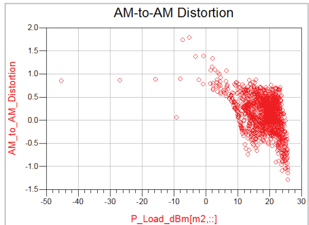
Figure 39. Plot of AM-to-AM distortion with a bias modulation waveform lag of 20 nsec.
