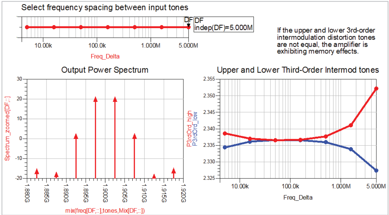
Figure 5. Simulation results for the example of a PA designed for wideband modulation.
