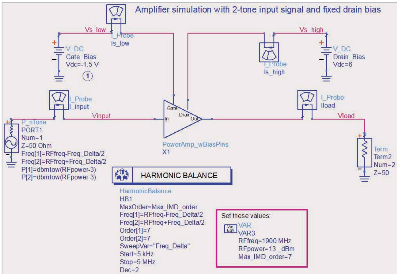
Figure 4. Simulation setup for a two-tone harmonic balance simulation.
