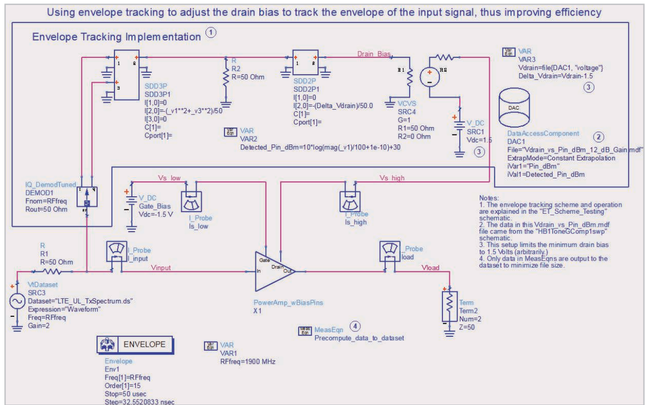
Figure 18. Schematic for using ET to adjust the drain bias.
