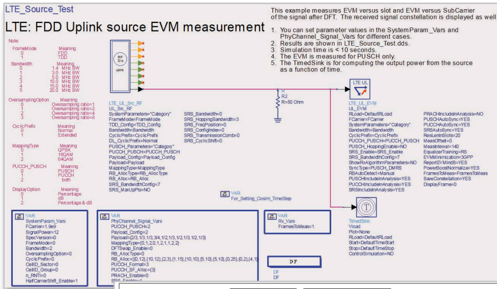
Figure 13. Setup for examining the ADS Ptolemy co-simulation source.
