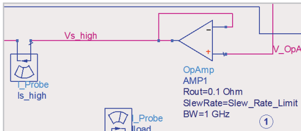
Figure 33. Schematic for modeling effects of a finite slew rate in the bias modulator.
