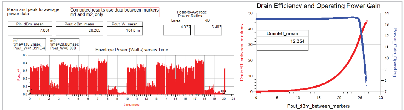
Figure 26. LTE_Cosim_Fixed_Bias_EVM_alt co-simulation results.
