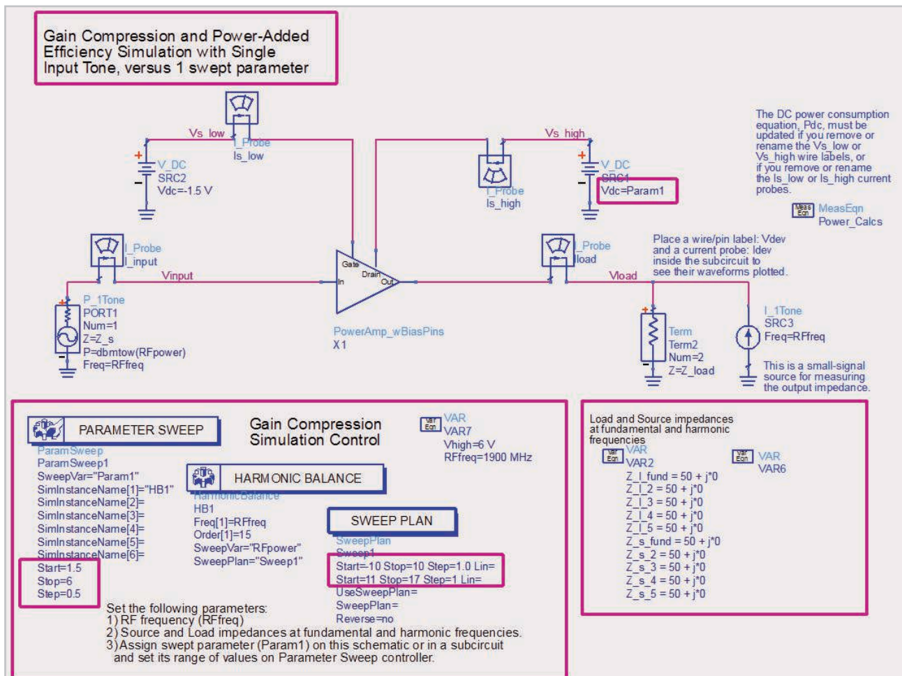
Figure 6. Simulation setup for characterizing the PA.
