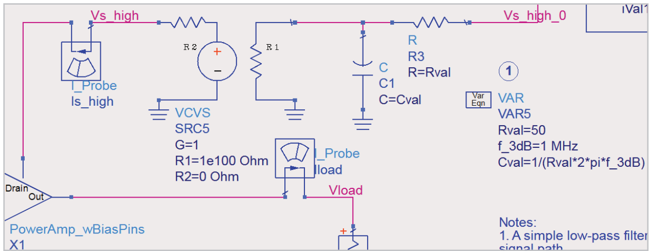
Figure 40. Schematic for simulating finite bandwidth in the bias modulation signal path.
