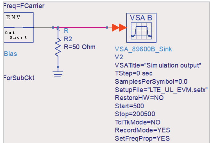
Figure 32. Simulation results are recorded on the VSA sink.
