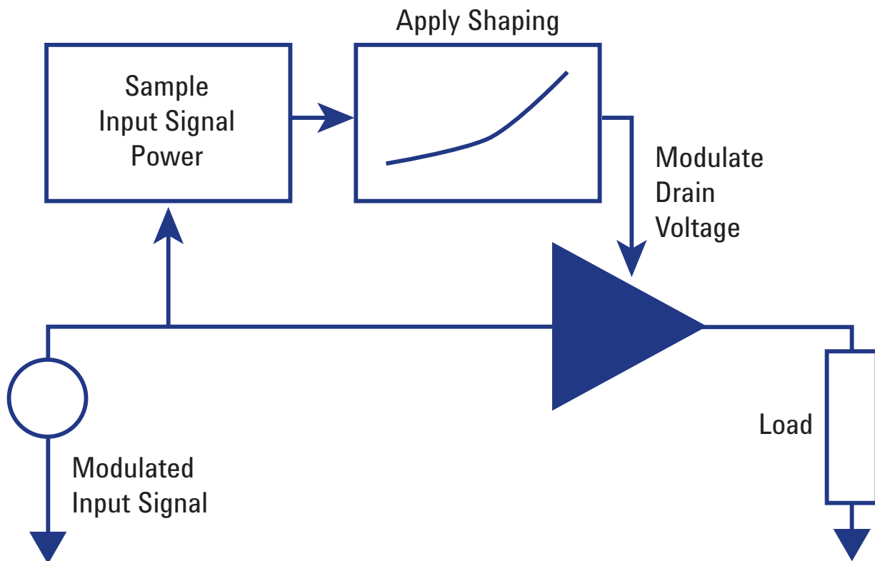
Figure 3. A block diagram for simulating Envelope Tracking.
